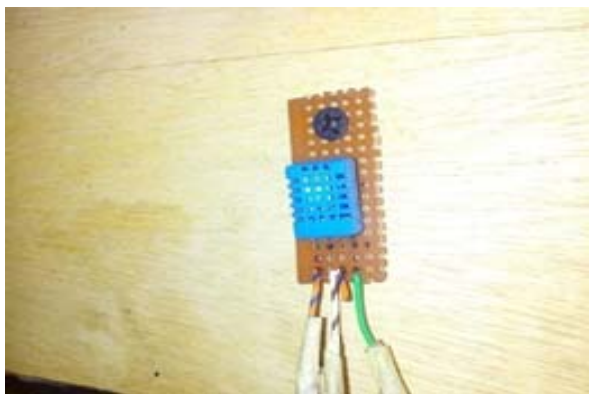
Plate 3: Sensor
