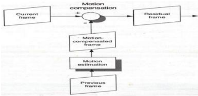
Fig 2: The Motion Compensator
