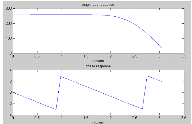
Fig 8: FIR Filter Response
