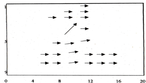
Fig 1: Motion Vectors
