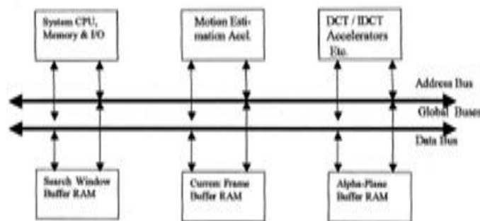
Fig 9: Video Encoder System Architecture
