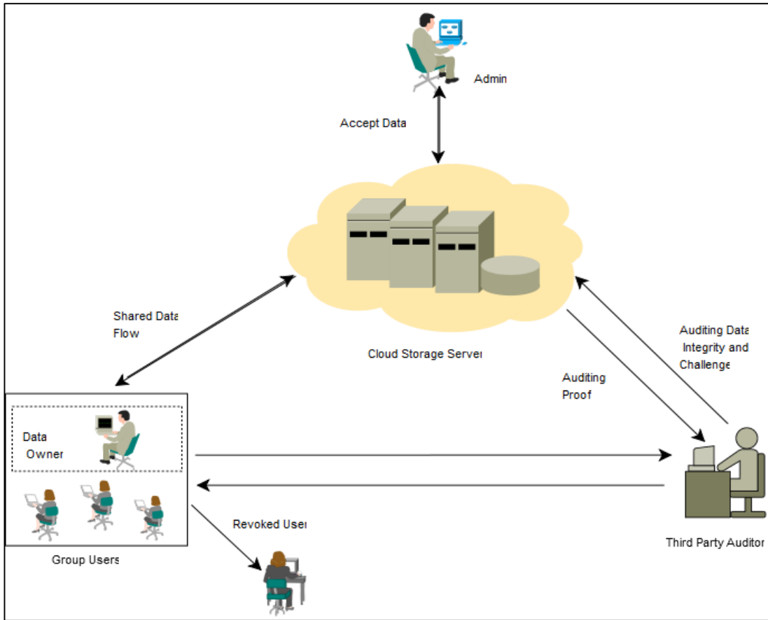
Fig 1: Architecture
